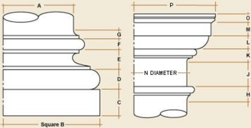
Doric Cap, Attic Base - No.105 Fluted
