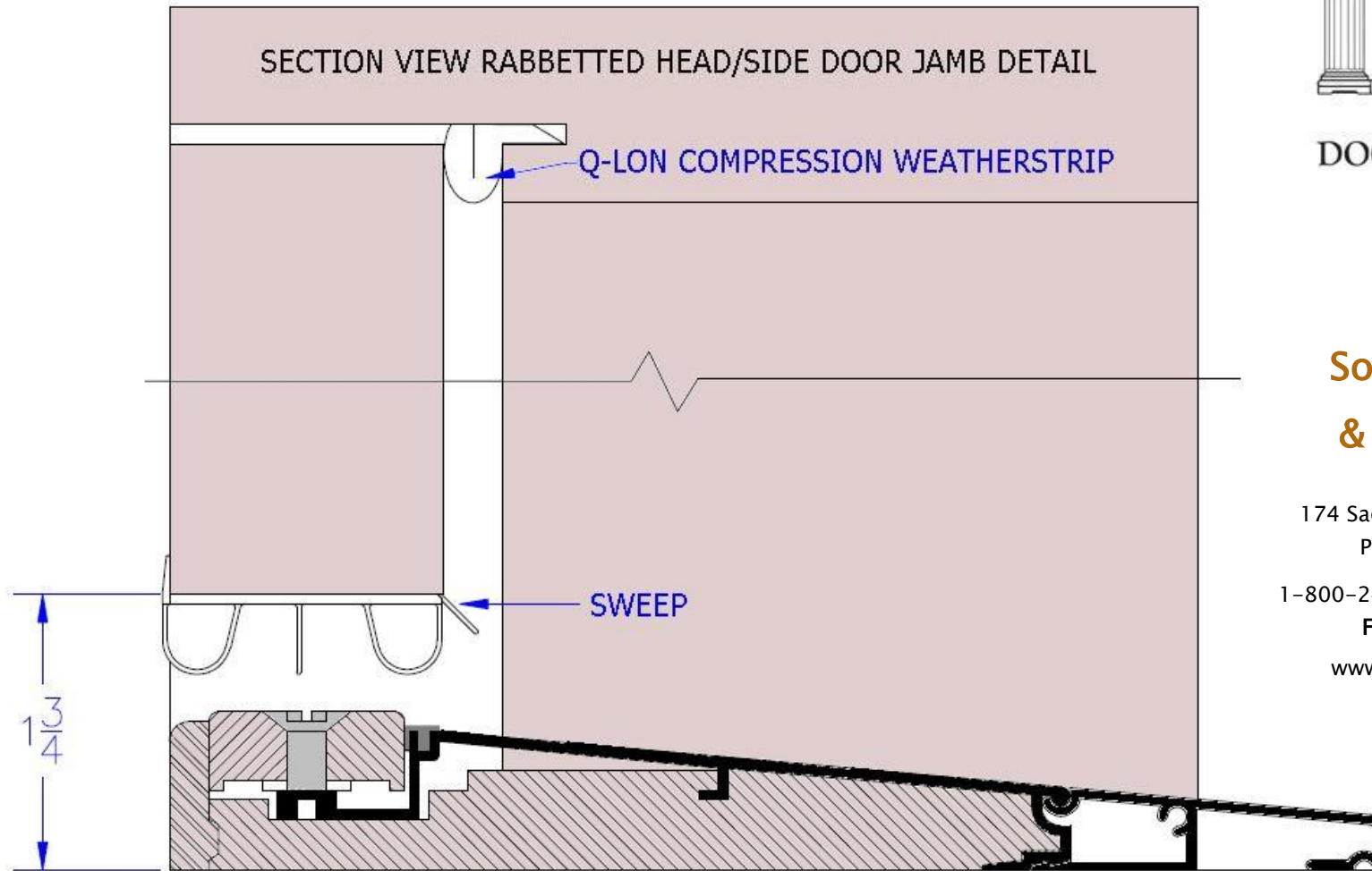
BRONZE ALUMINUM ADJUSTABLE SILL WITH EXTENSION
